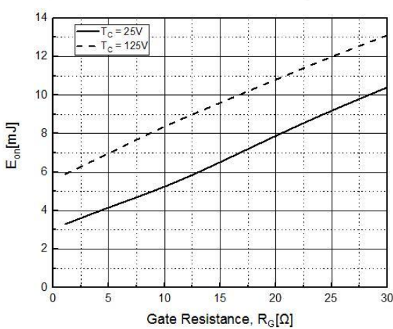
Fig. 5. Turn-on Characteristics vs. R_G
