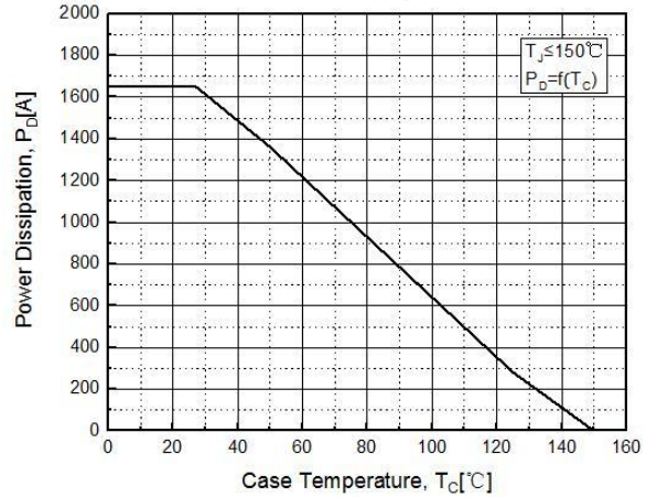
Fig. 8. Power Dissipation vs. T_c
