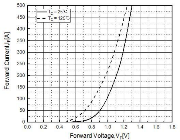
Fig. 10. Forward Characteristics
