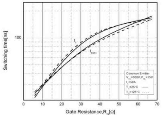
Fig. 6. Turn-on Characteristics vs. R_G
