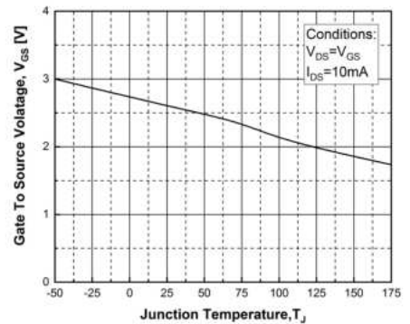
Fig. 6. Threshold Voltage vs. Temperature
