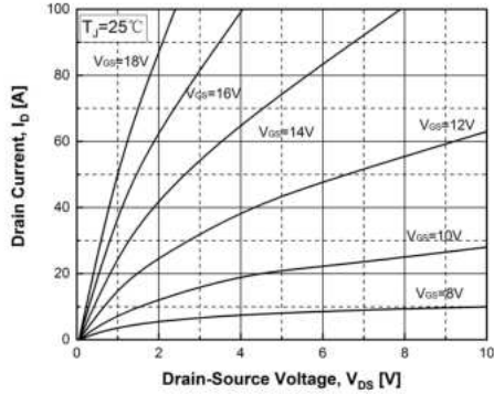
Fig. 1. Typical on-Resistance Characteristics T J =25°C
