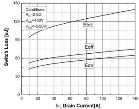
Fig. 12. Typ. Switching losses vs. Drain current
