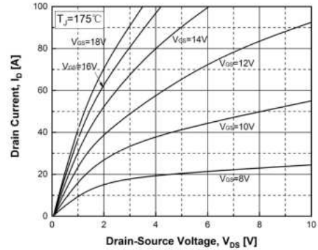
Fig. 2. Typical on-Resistance Characteristics T J =175°C
